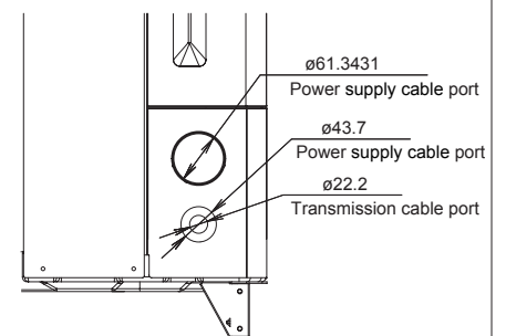
B Left side knockout position
