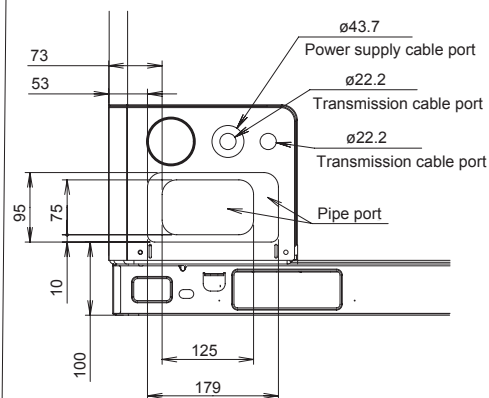
A Front side knockout position
